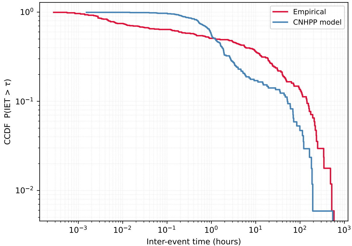
User 32432053 - Empirical vs CNHPP model
